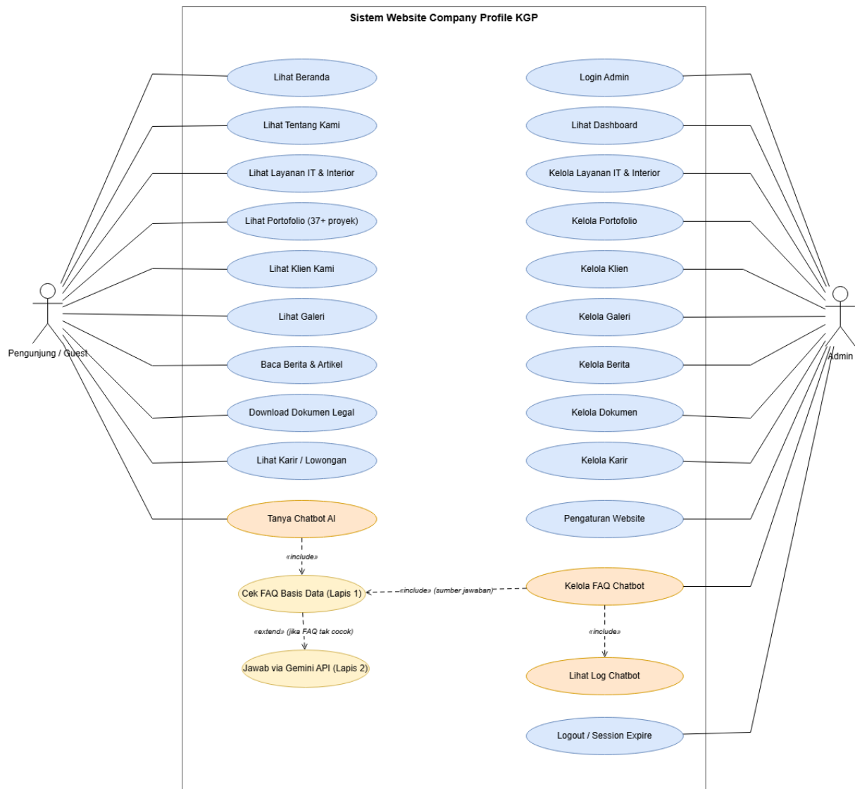
Gambar 2. Use Case Diagram (UML) — Web Company Profile KGP
